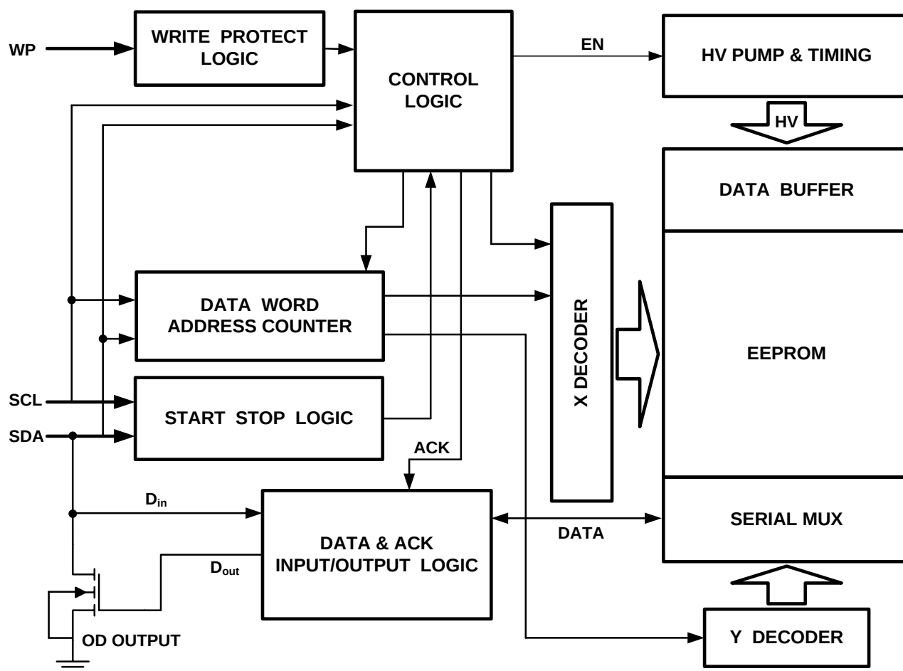
Figure 1. Block Diagram
